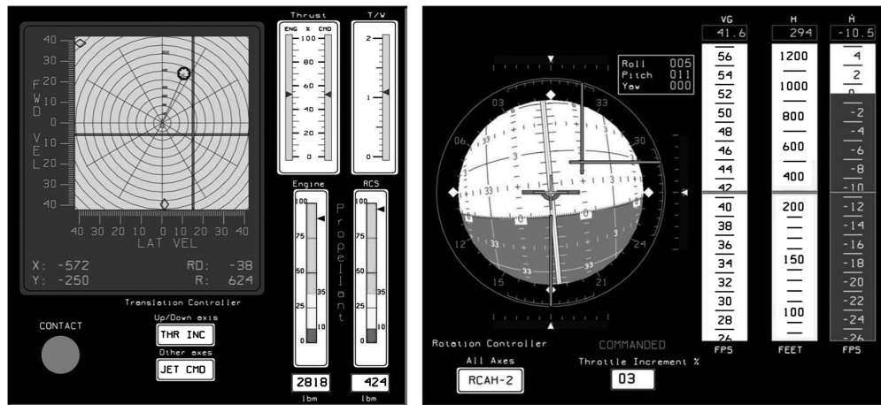
Fig. 5 Pilot station displays.
