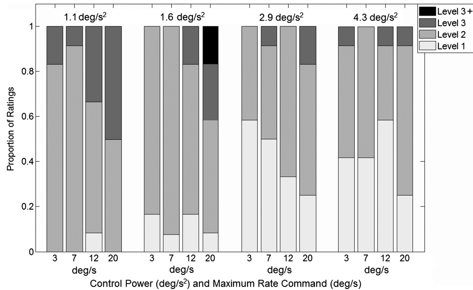
Fig. 6 Proportion of HQ levels for the 16 primary configurations.
