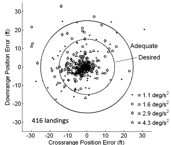
Fig. 10 Range to target point at touchdown.
