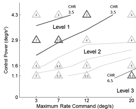
Fig. 8 Cross plot of median CHRs.
