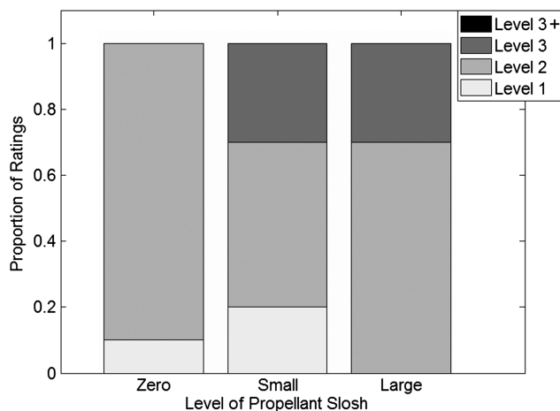
Fig. 14 Proportion of HQ levels with propellant slosh for 1.6 deg/s 2 and 7 deg/s.
