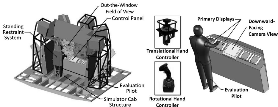
Fig. 4 Simulator cockpit layout.
