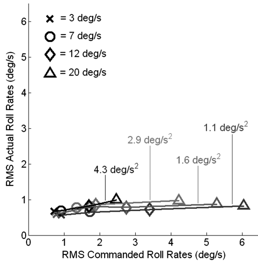
Fig. 13 RMS commanded and actual roll rates.
