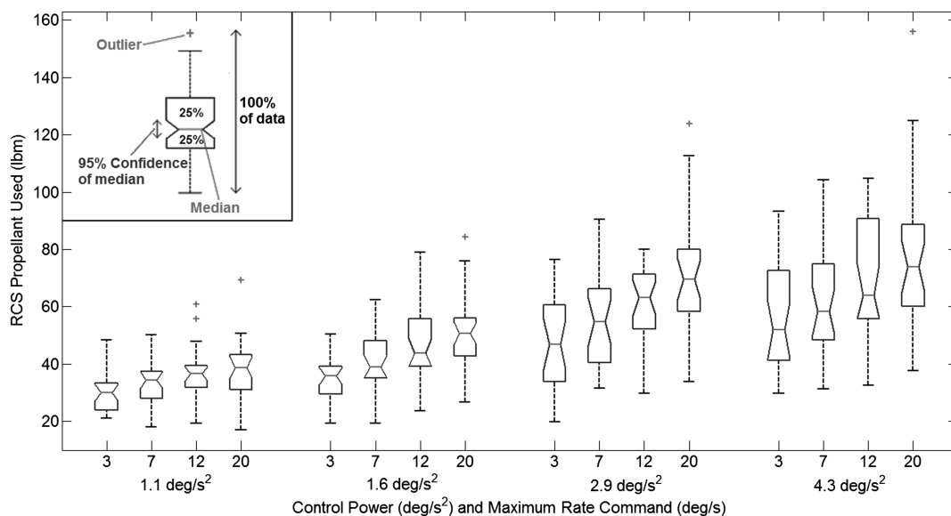
Fig. 12 RCS propellant used.
