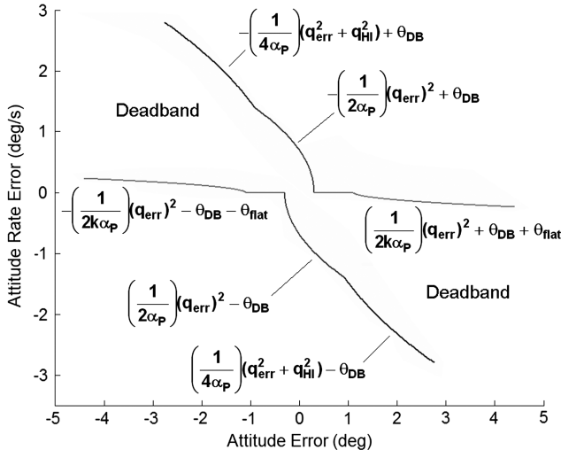
Fig. 3 Switching curves for pseudoautomode.
