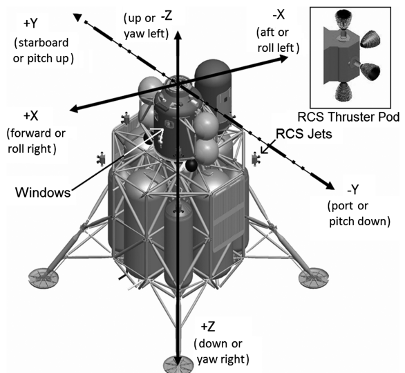
Fig. 2 Schematic of lander design.
